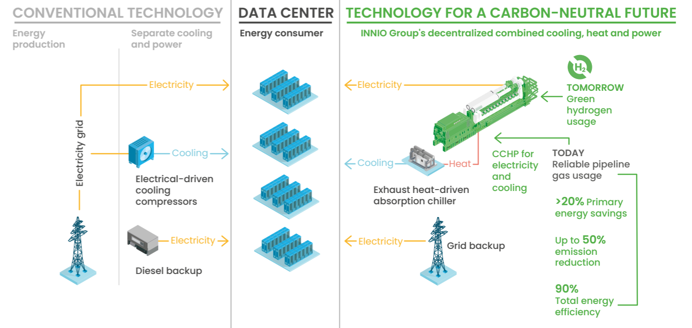
Figure 12: H 2 engine-based CCHP concept for data centers
